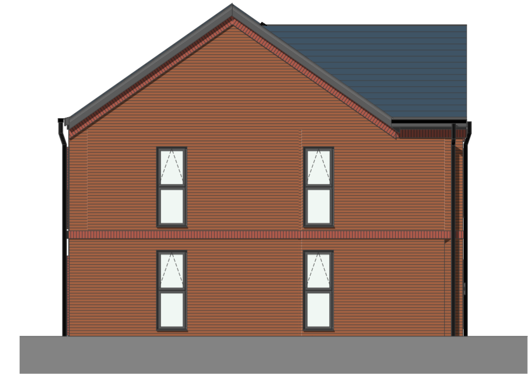
Block 01 Proposed West Elevation 1:100
