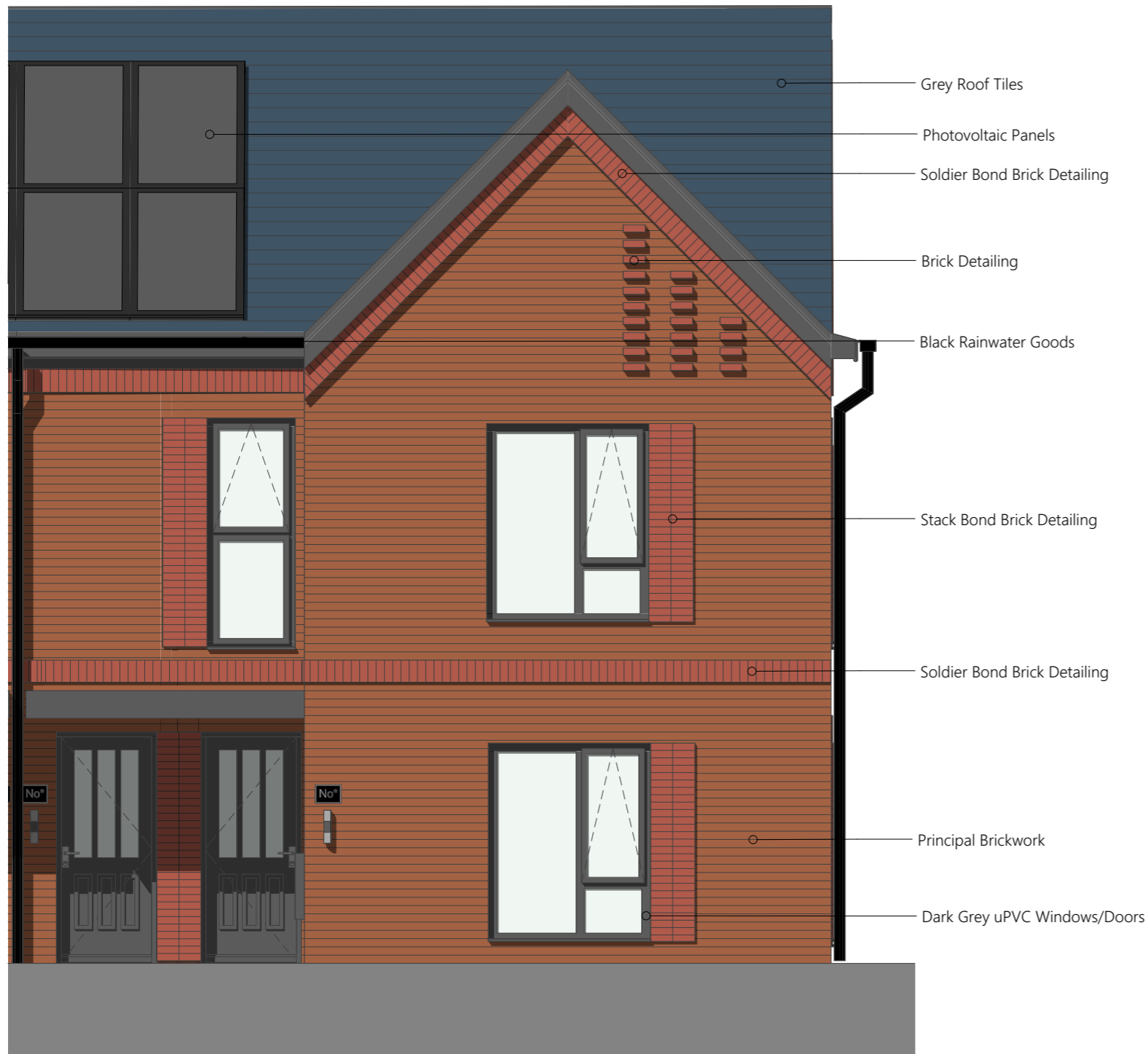
Proposed Front Elevation (Block 04 & 09)
