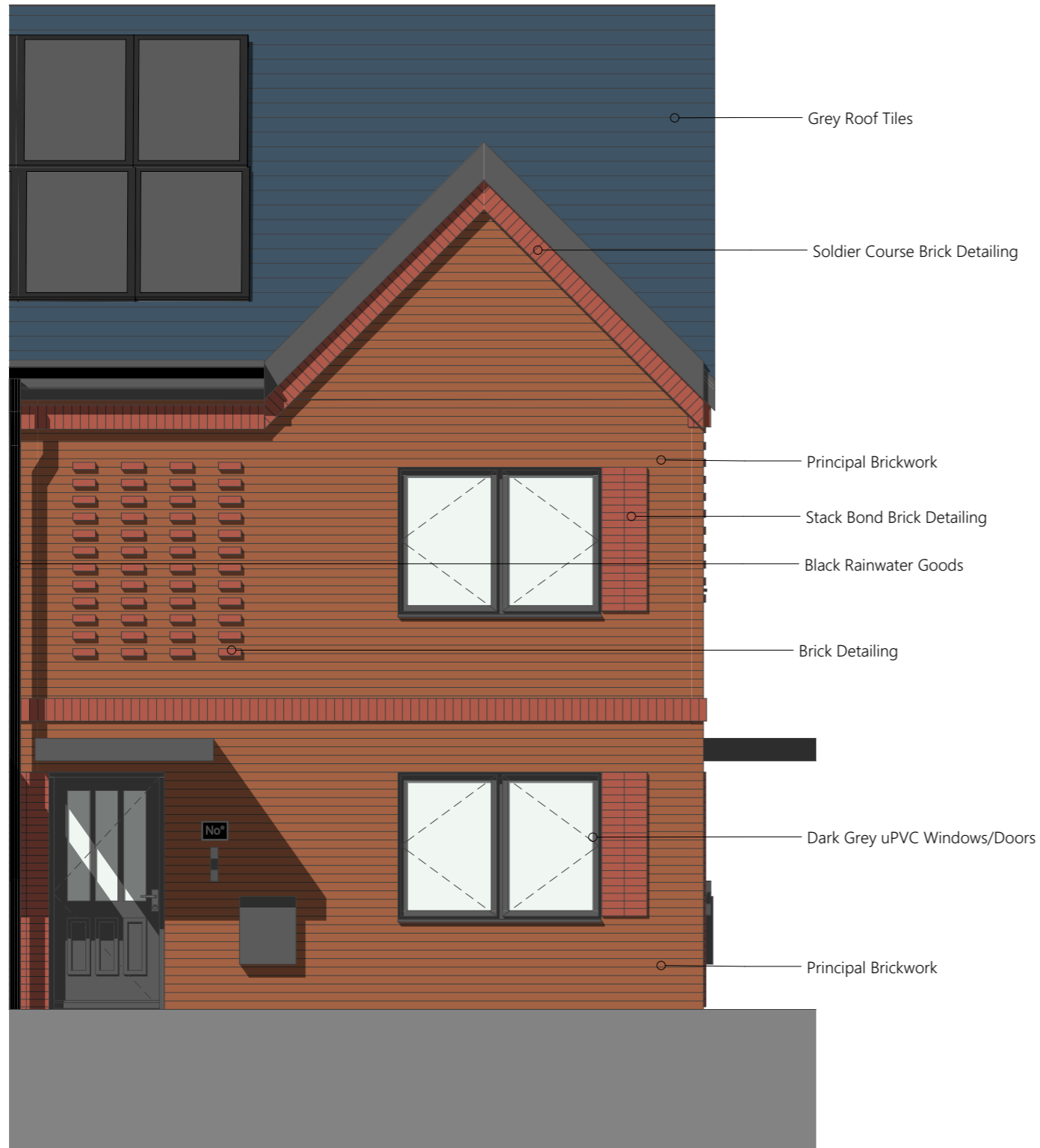
North Site Blocks 02 & 03 Front Elevation 1:50
